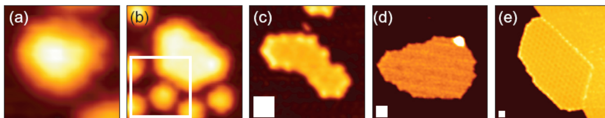
Figure 8. STM topographs of typical graphene islands prepared with the TPG procedure on Ir(111), after annealing for 20 s to (a) 598 °C, 3.2 nm \times 3.2 nm, (b) 697 °C, 6.2 \times 6.2 nm, (c) 847 °C, 18 nm \times 18 nm, (d) 1047 °C, 32 nm \times 32 nm and (e) 1197 °C, 64 nm \times 64 nm. The size of the white box corresponds to the size of the smallest topographic image (3.2 nm \times 3.2 nm). The islands undergo a transition from an undefined, probably amorphous state to a compact shape at low temperature to non-compact shapes at intermediate temperature and (c) back to more compact shapes at high temperature (reproduced from [52]).
