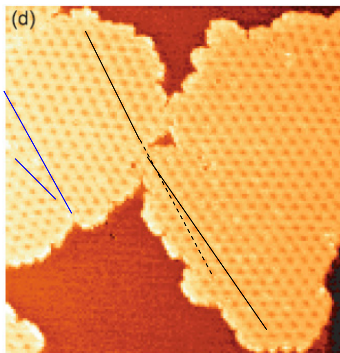
Figure 9. STM topograph ( 70\text{ nm} \times 73\text{ nm} ) of graphene grown by CVD on an Ir(111) surface at 847^\circ\text{C} , out of exposure to an ethene partial pressure of 5 \times 10^{-10}\text{ mbar} , for 20 s; two coalesced islands forming a coherent graphene island; the misorientation is evident from the deviation in the orientation of the rows of minima in the STM images (highlighted with black lines). Note that the left-hand side island, in fact, is composed of two different islands with differing orientations (highlighted by blue lines) (adapted from [52]).
