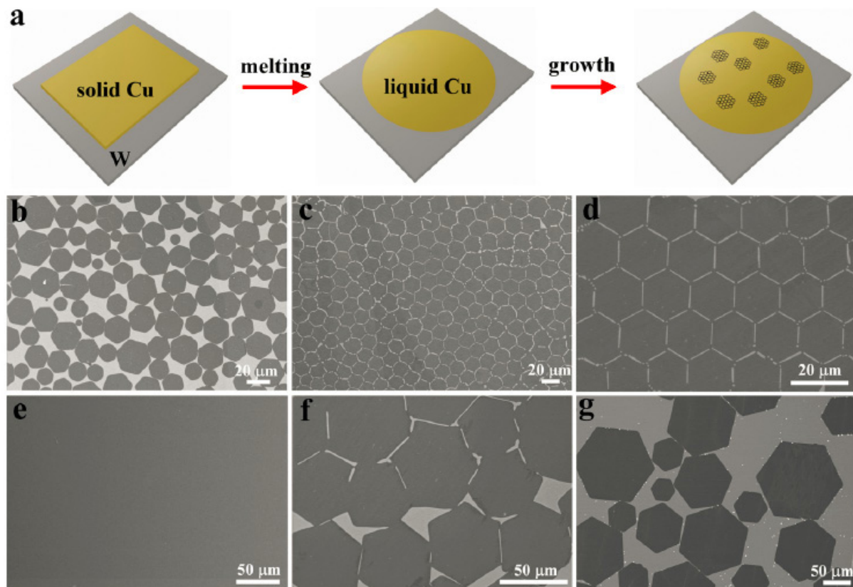
Figure 13. The growth of HGFs on flat liquid Cu surfaces on W substrates. (a) Scheme showing the CVD process for the synthesis of HGFs on a liquid Cu surface. (b) SEM image showing partially covered and well-dispersed HGFs using 6 sccm \text{CH}_4 /300 sccm \text{H}_2 at 1120^\circ\text{C} for 30 min. (c) SEM image of HGFs showing a compact assembly of HGFs in which the dark and bright parts represent HGFs and the Cu surface, respectively. (d) SEM image of a near-perfect 2D lattice composed of similar-sized HGFs. (e) SEM image of the sample for 2 h growth showing the continuous graphene film with uniform contrast. (f) and (g) SEM images of large-sized HGFs showing that the average sizes are approximately 50 and 120\ \mu\text{m} using 1140^\circ\text{C} and 1160^\circ\text{C} , respectively. Experimental conditions from (c) and (d) are the same, using 6 sccm \text{CH}_4 /300 sccm \text{H}_2 at 1120^\circ\text{C} for 38 min (reproduced from [73], copyright (2012) National Academy of Sciences, USA).
