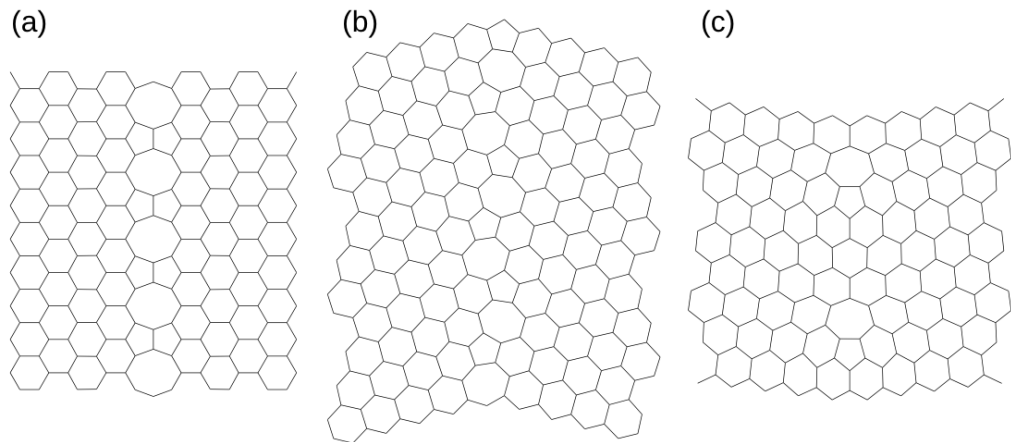
Figure 2. Examples of ordered GBs. All the models shown in this figure were relaxed with the Brenner–Tersoff potential. (a) Two translated graphene half sheets with parallel zigzag edges (no tilt angle) interconnected through alternating pentagon pairs and octagons [32]. (b) Grain boundary realized with adjacent pentagon–heptagon pairs, obtained by joining two grains with edges parallel to the direction (1, 3) relative to the same set of lattice vectors \mathbf{a}_1 and \mathbf{a}_2 as in figure 3 (misorientation angle \tau = 27.8^\circ ). (c) Grain boundary with index (3, 2) in the notation of [20], with misorientation angle \tau = 46.8^\circ , shaped into a linear chain of pentagon–heptagon pairs separated by three transverse rows of hexagons.
