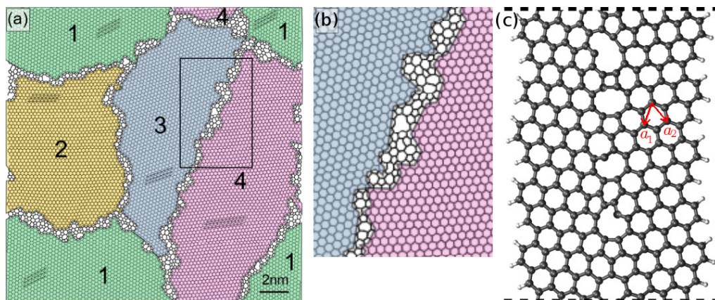
Figure 1. Examples of disordered GBs. (a) Polycrystalline graphene generated on the computer in a 20 \times 20 nm box with periodic boundary conditions in the two directions (reproduced from [21], copyright (2012) by the American Physical Society). Zigzag directions in each grain are marked by sets of parallel lines. (b) Zoom of the area delimited by the rectangle drawn across the boundary between grains 3 and 4 in panel (a). (c) Boundary between two half-ribbons with thermally disordered (9,5) edges relative to the basis vectors shown by red arrows, the structure being saturated with hydrogen on its free edges and reproduced periodically along the vertical direction (adapted from [30]).
